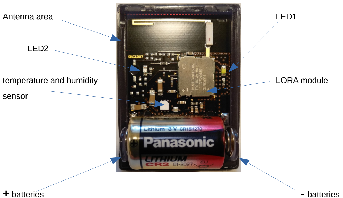
iNode LORA HT – view after removing the cover
